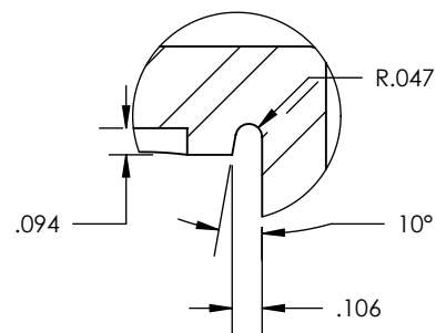
DETAIL B SCALE 2 : 1.5
