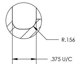
DETAIL C SCALE 2 : 1.5
